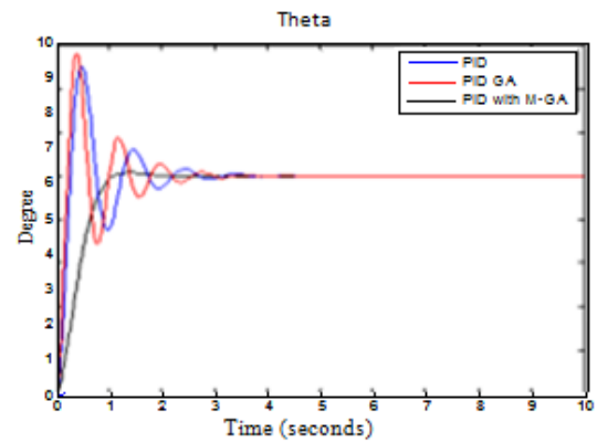
Fig. 9. Comparison of results for Pitch (Theta)
