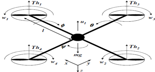
Fig.1. Theoretical Model of Quadcopter
